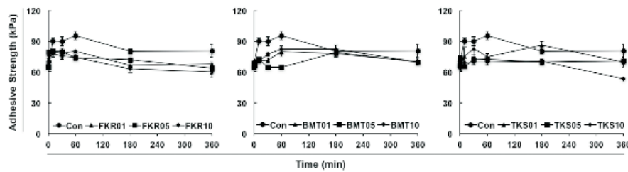
Figure 5. Variations in adhesive strength.
